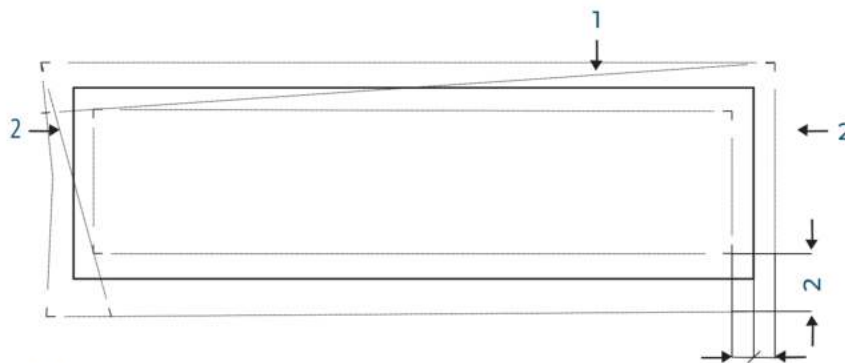
Figure 5 - Example of tolerances on angles.
