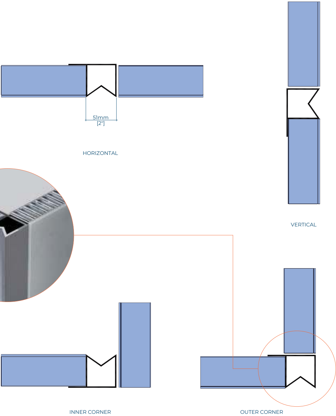
OPTION 6: FACE ALIGNMENT (A6)
