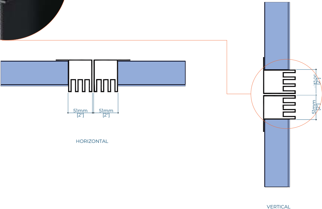
OPTION 13: FACE PROTRUDED (A13P-A13P)
