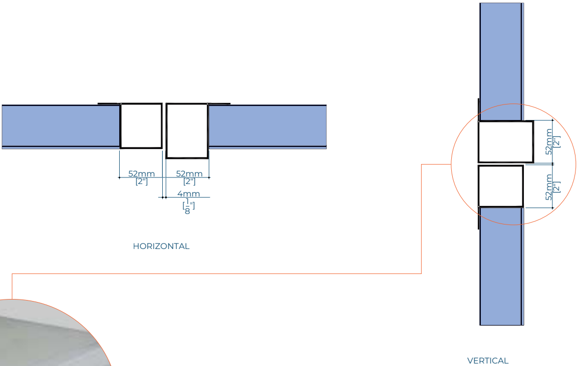
OPTION 14: FACE ALIGNMENT (A1-A1P)
