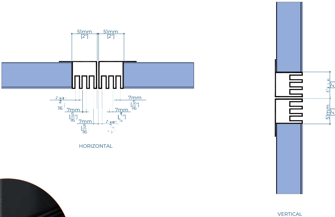
OPTION 13: FACE ALIGNMENT (A13-A13)
