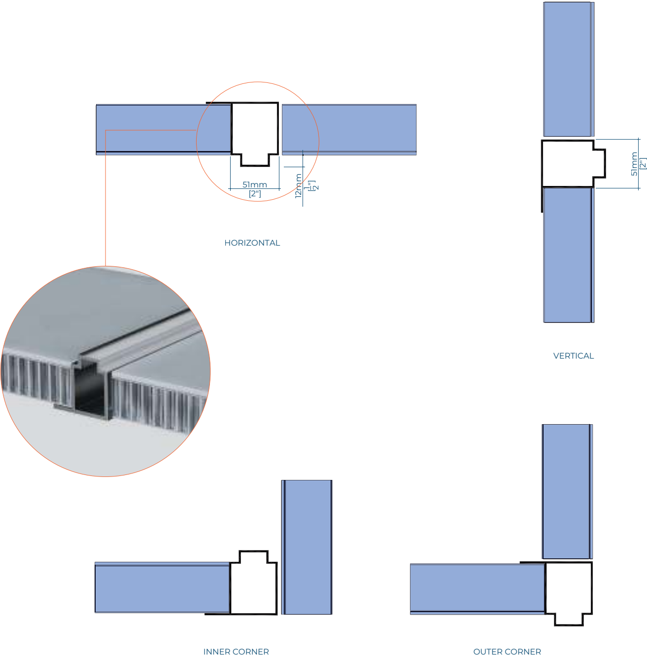
OPTION 8: FACE ALIGNMENT (A8)
