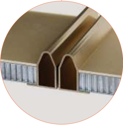
OPTION 12: FACE PROTRUDED (A12P-A12P)
